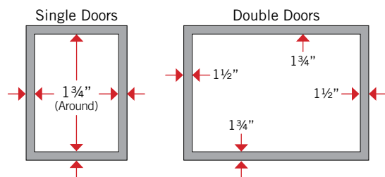
Flange Overlap Dimensions / Legacy Doors
