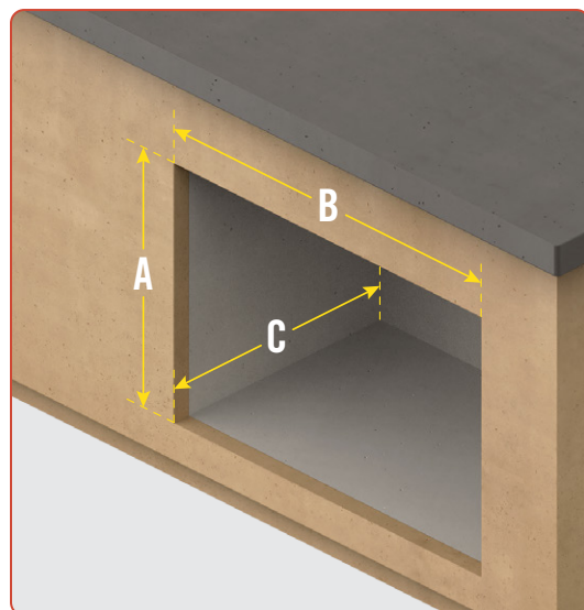
Flange Overlap Dimensions / Select Doors
