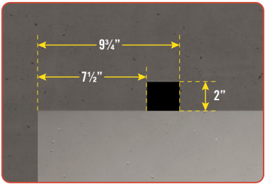
Detail #2: For Beverage Butler.
