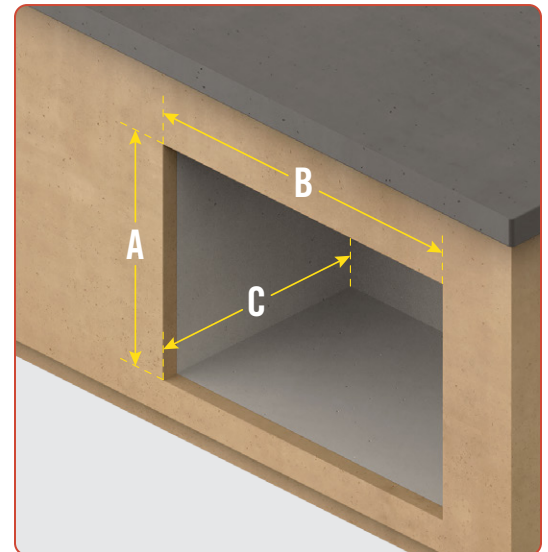
Flange Overlap Dimensions / Premium Flush Doors
