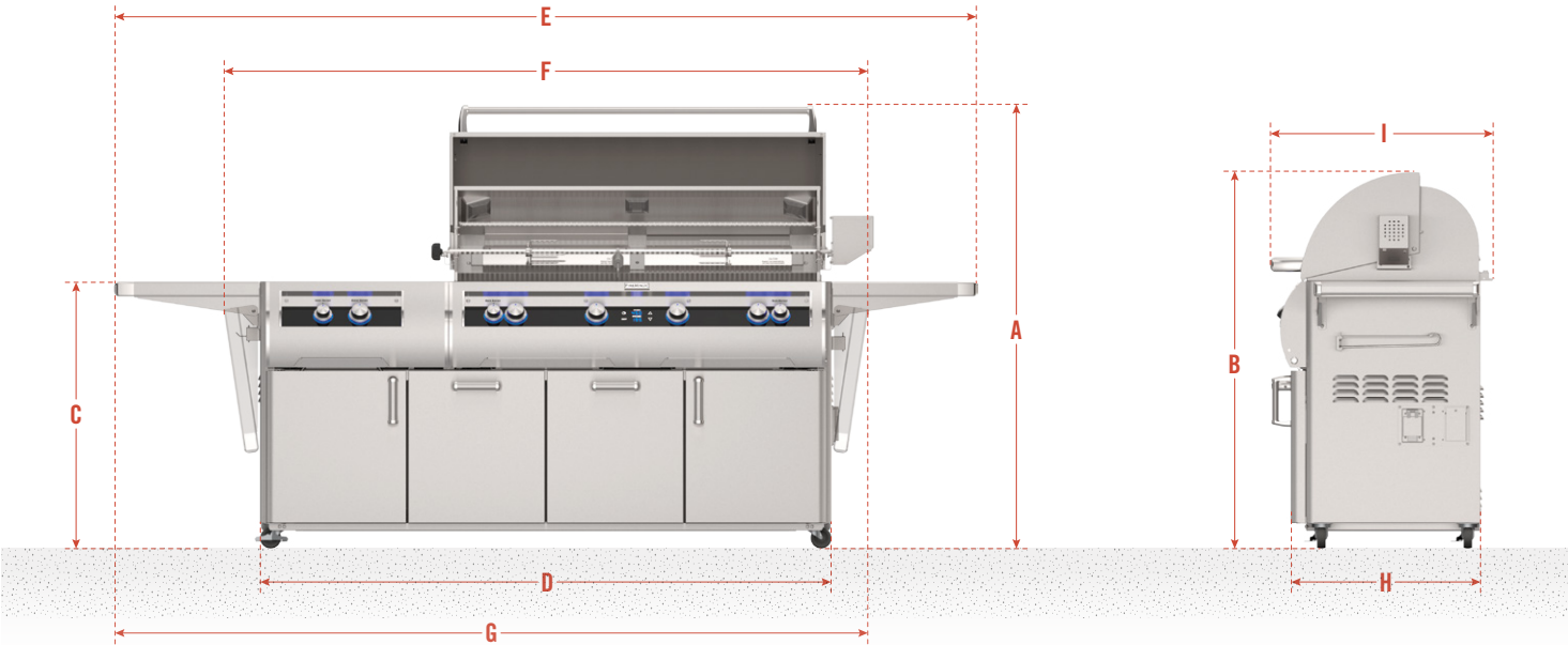
General Dimensions - E1060s 52" Portable Grill
