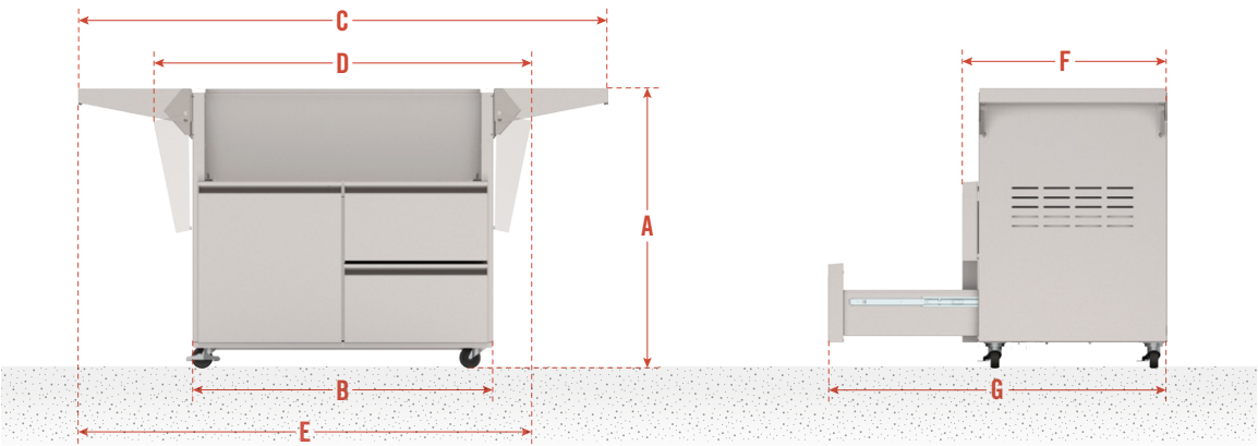
General Dimensions - Portable Cart Bases
