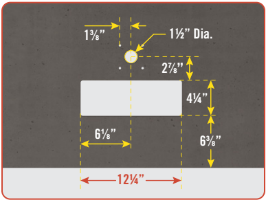
Detail #1: For Outdoor Kegerator.
