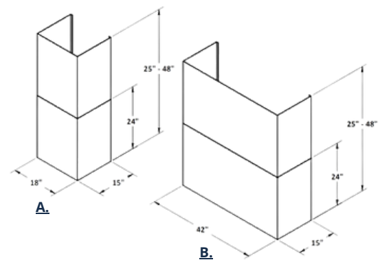
DUCT COVERS: MODEL #: A. DC7200S; B. DC7200D
