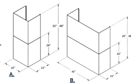
DUCT COVERS: MODEL #: A. DC7200S; B. DC7200D
