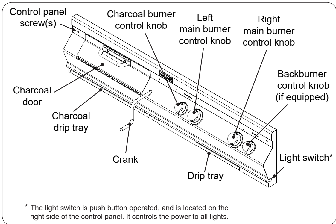
Fig. 35-1 A830 controls
