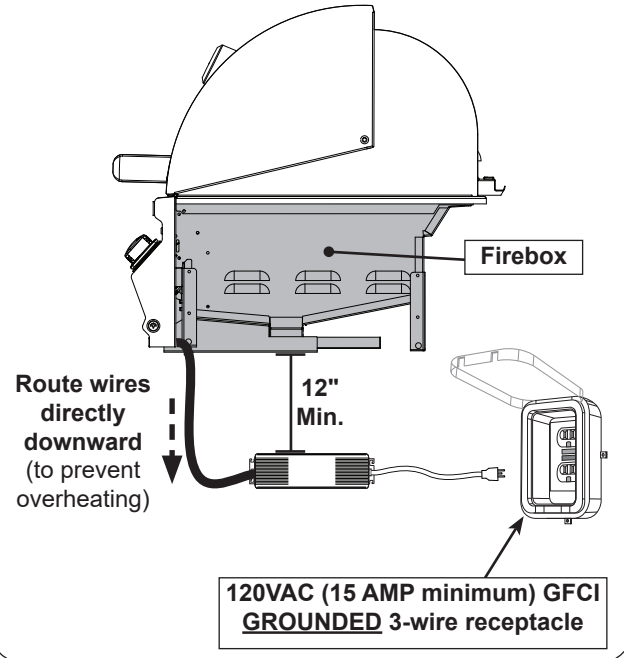
Fig. 29-1 Electrical installation
