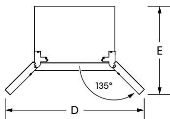
TOP VIEW (DOORS OPENED)
