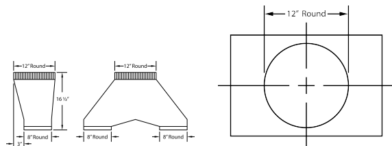
VP563 Transition (Optional) For B400 (Double B200 Dual Blowers)
