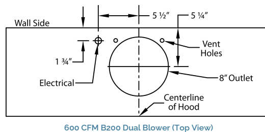
600 CFM B200 Dual Blower (Top View)
