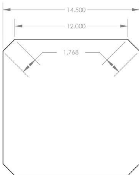
SNK-15D / SSKN-15D ISLAND TOP VIEW CUTOUT DIMENSIONS
