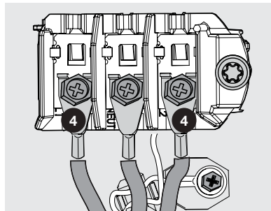
4 Outer Brass Terminals
