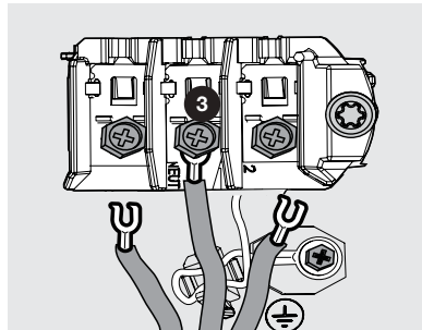
3 Neutral Silver Terminal
