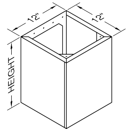
Wall Mount Duct Cover Models: WDCRND-12/12, WDCRND-12/24, WDCRND-12/36
