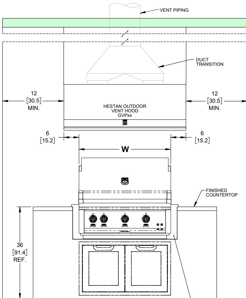
FRONT VIEW
