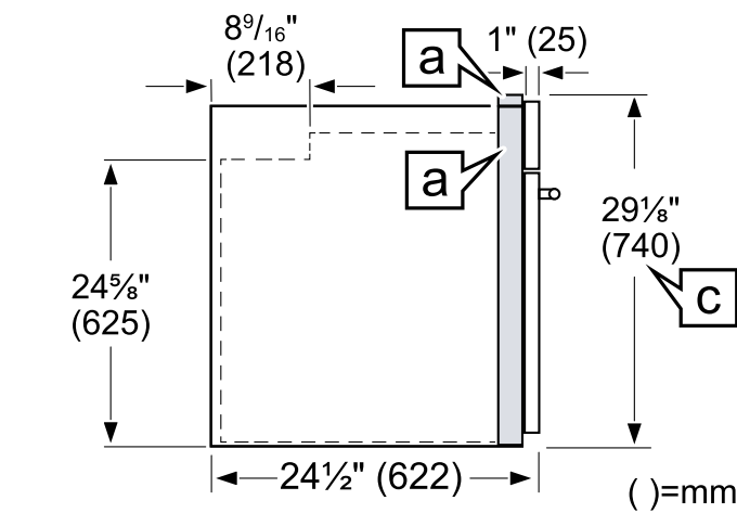
Side view (representative)
