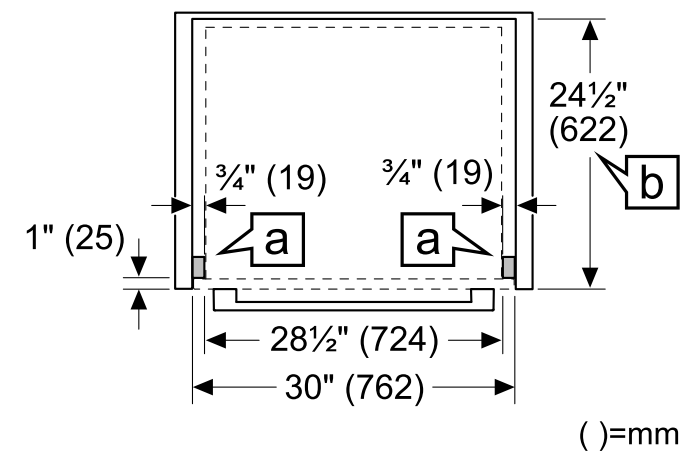
Top view bottom hinged door
