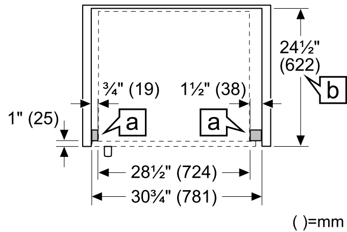
Top view right swing door
