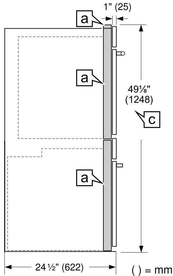
Side view
