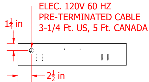
SIDE VIEW (OPEN)
