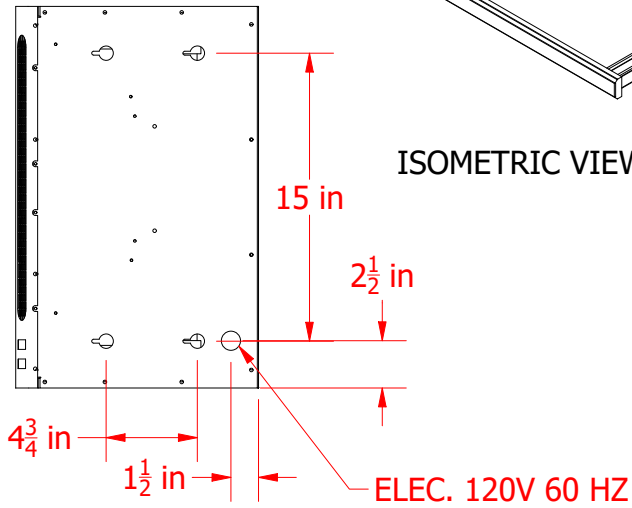
TOP VIEW (CLOSED)
