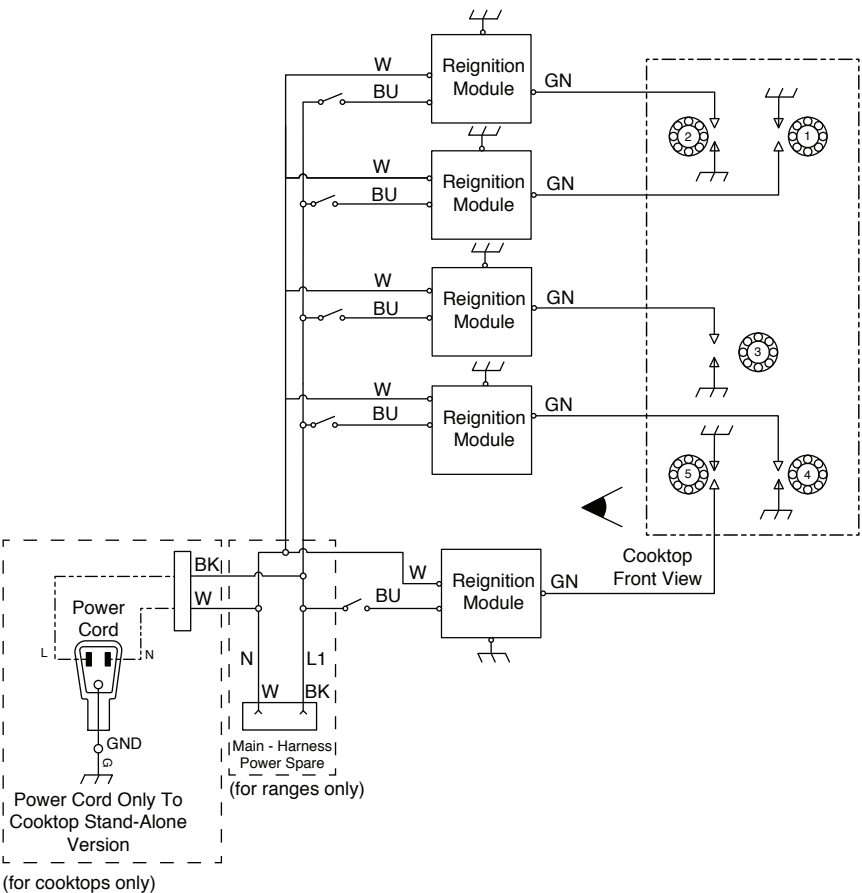
5 Burner Cooktop
