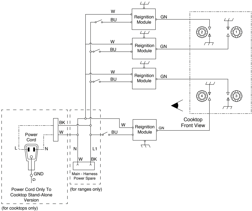
4 Burner Cooktop
