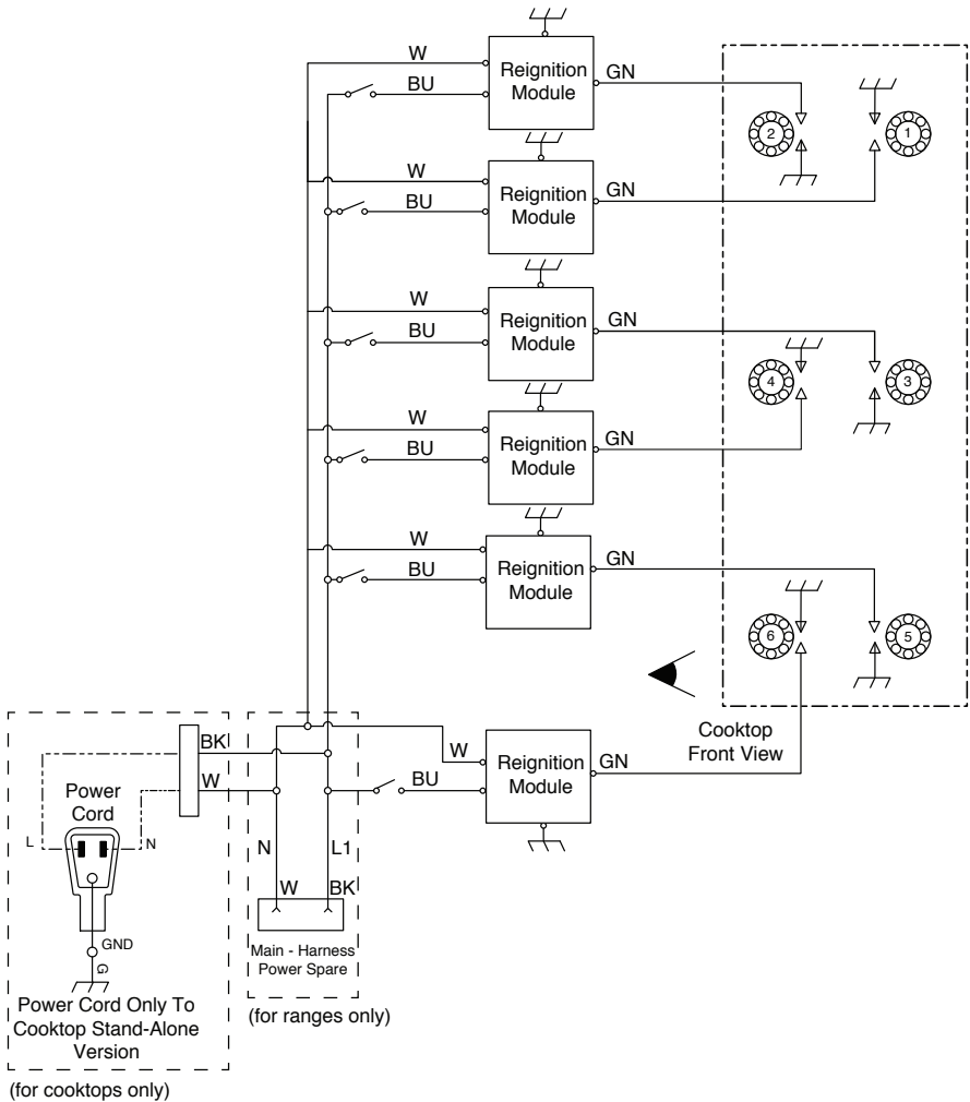
6 Burner Cooktop
