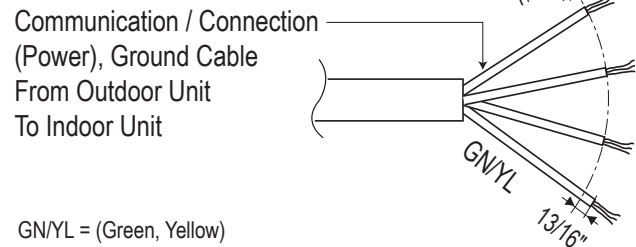
Figure 52: Single Zone Outdoor Unit to Indoor Unit Wiring and Communications Cable Diagram.
