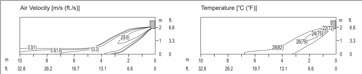
Figure 18: Mega 115V KNSAC091B Air Velocity and Temperature Distribution Charts.
