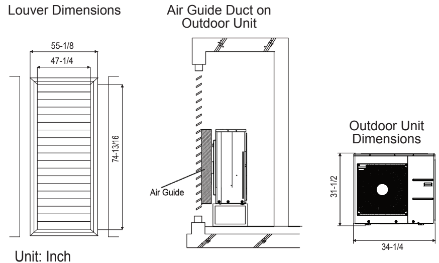
Figure 36: Example of Installing Outdoor Unit Indoors.
