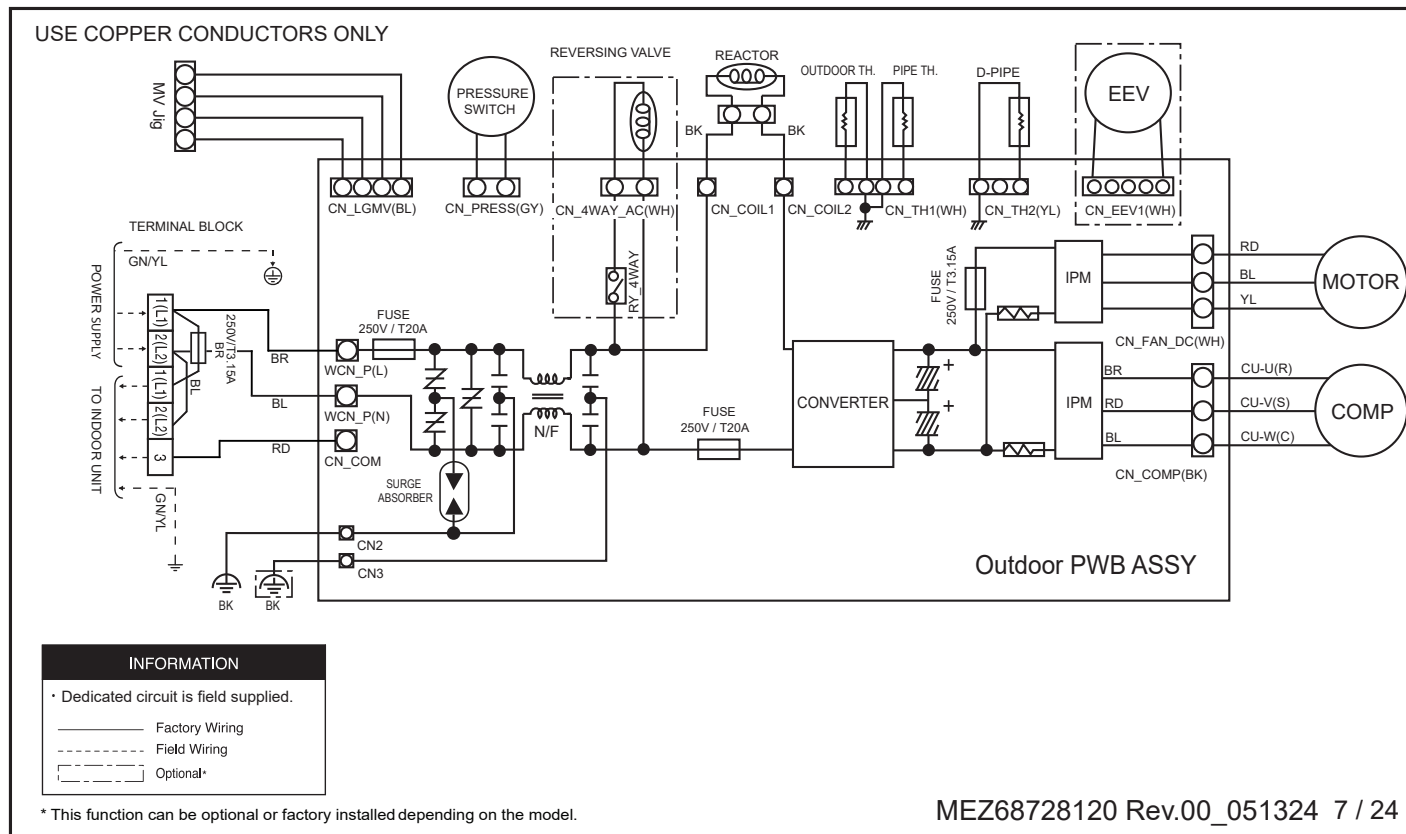
Figure 48: Mega 115V KUSAC091B and KUSAC121B Outdoor Unit Wiring Diagram.
