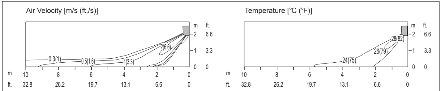
Figure 19: Mega 115V KNSAC091B Air Velocity and Temperature Distribution Charts, continued.
