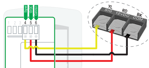
Figure 58: Example of Wired Controller Terminals.
