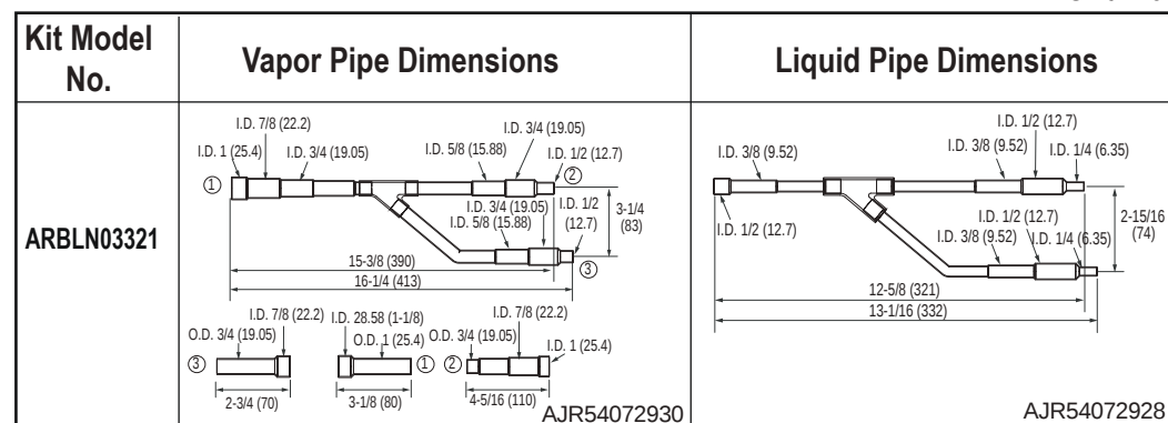
Figure 29: Indoor Unit Y-Branch Dimensions.
