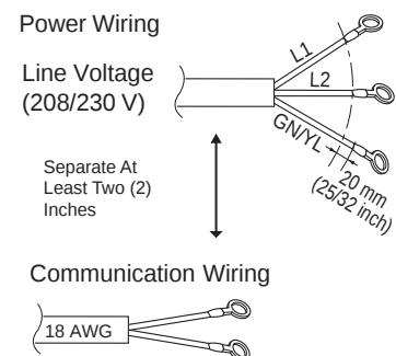
Figure 35: Power Wiring and Communication Wiring from ODU to IDU / BDU (Multi F MAX with LGRED Only), and from the BDU to the IDU (Multi F MAX with LGRED Only) GREATER THAN 130 feet.
