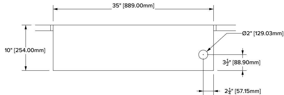
FRONT
