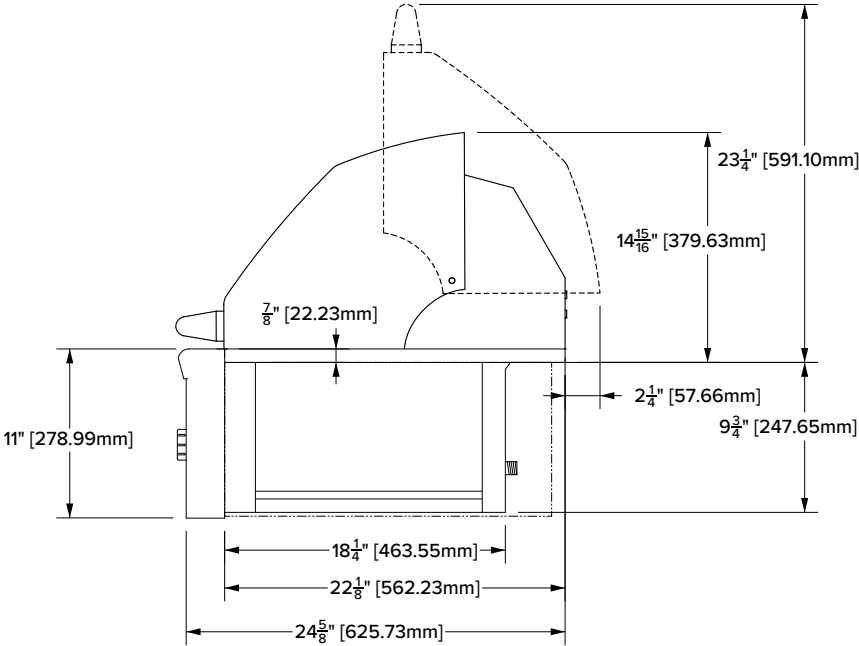
SIDE
