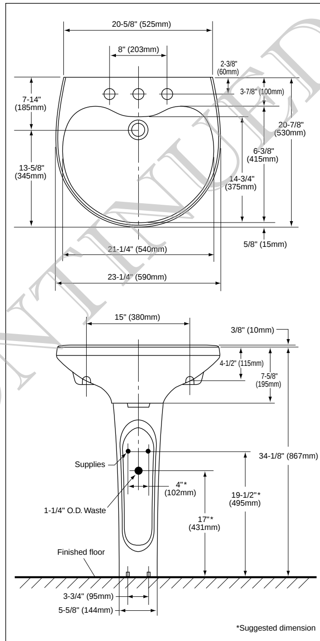
LPT630.8N - Lisette Pedestal Lavatory
