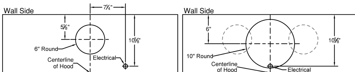
M600 &amp; M1200 Connection Diagrams
