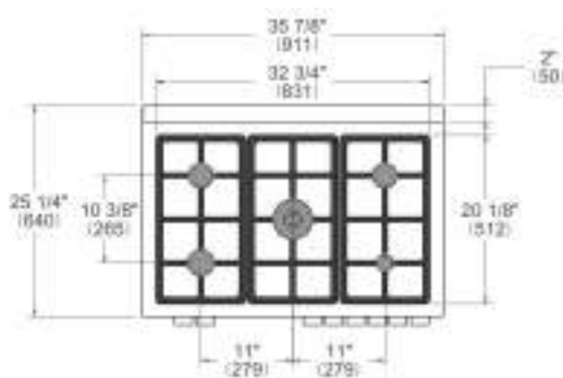
WORKTOP DETAILS
