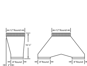
VP563 Transition (Optional) For B400 (Double B200 Dual Blowers)
