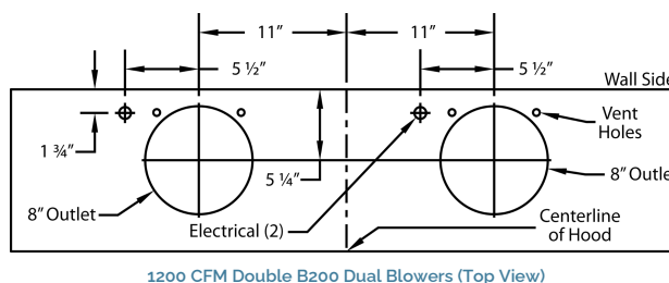
1200 CFM Double B200 Dual Blowers (Top View)
