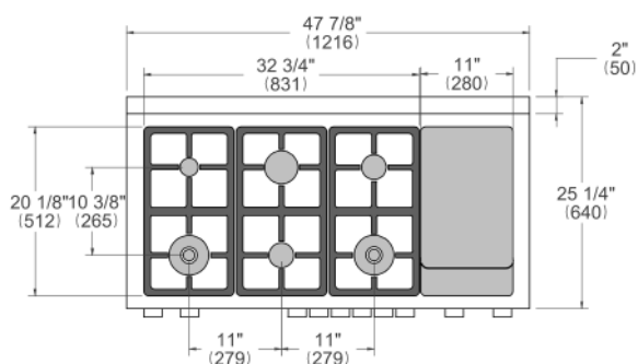
WORKTOP DETAILS
