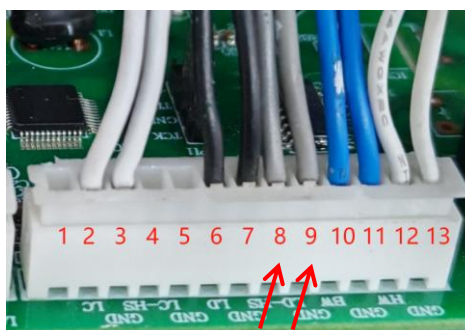
F5 Test points
