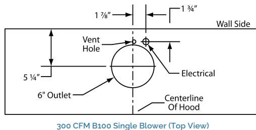
300 CFM B100 Single Blower (Top View)
