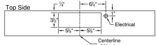
(Wall Cutout, Viewed from Front)
