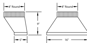
VP565 Standard Transition (Included)
