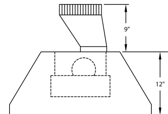
Transition Installed (Side View)
