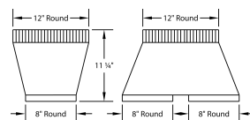
VP564 Standard Transition (Included)
