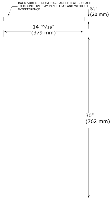
Integrated Panel
