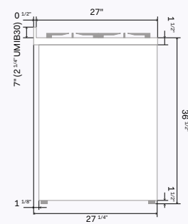
Side view UM30
