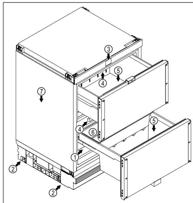
Fig. 1 Exemplary illustration of the front side
