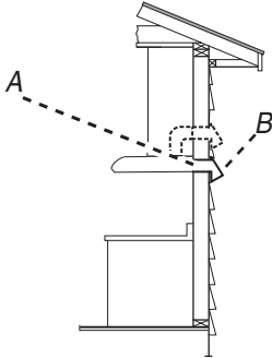
A. 3¼" x 10" (8.3 x 25.4 cm) rectangular vent through the wall or out the top (purchased separately). B. Wall cap with damper (purchased separately)
