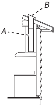
A. 3¼" x 10" (8.3 x 25.4 cm) rectangular vent through the roof (purchased separately). B. Roof cap with damper (purchased separately)
