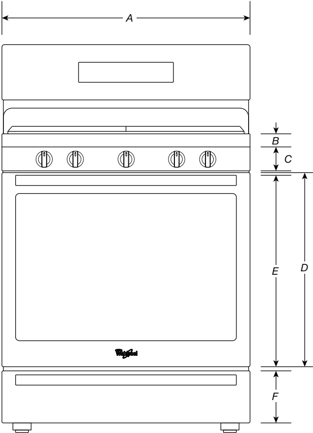
VISTA FRONTAL
