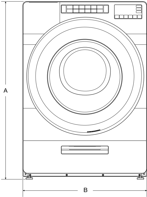
VISTA FRONTAL
