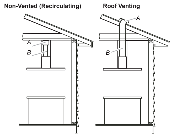
A. Deflector A. Roof cap B. 6" (15.2 cm) round vent B. 6" (15.2 cm) round vent
