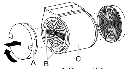
A. Charcoal Filter
